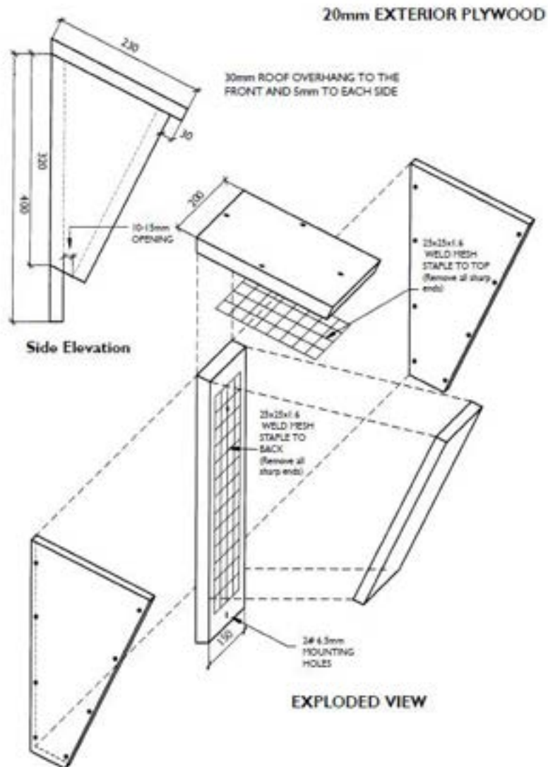
Figure 111. Design for construction of microbat roosting habitat box (Ipswich City Council, 2009)
